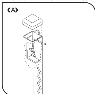
ATTACHING THE NET TO FIXED END POST
