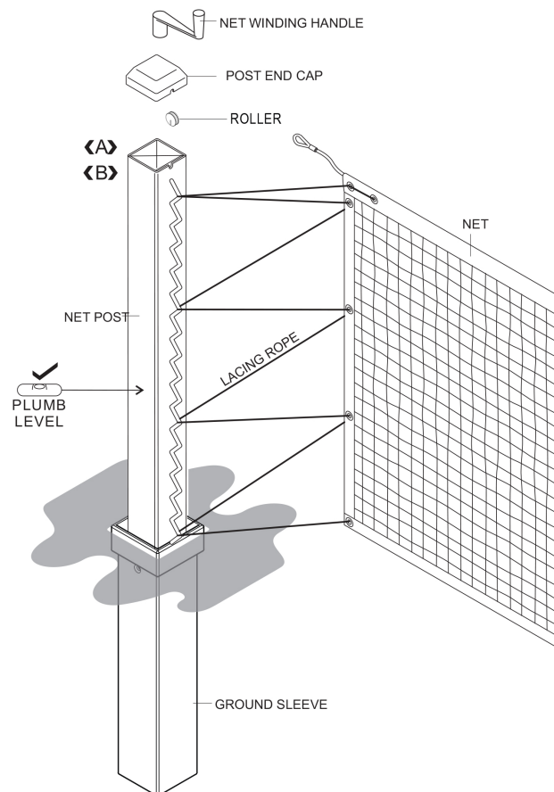
ATTACHING THE NET TO FIXED END POST
