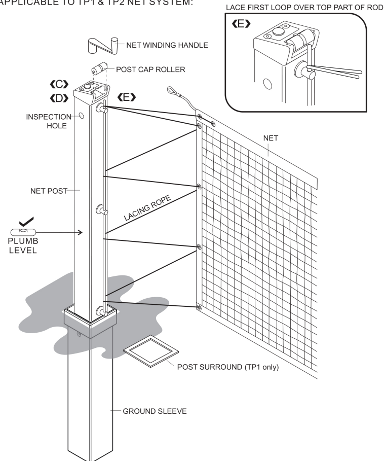
ATTACHING THE NET TO FIXED END POST
